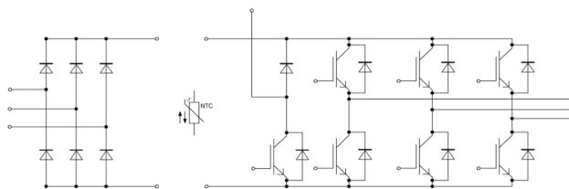
Internal Circuit
