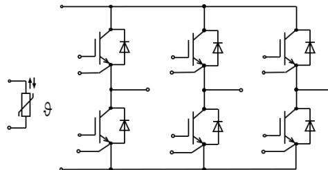
Internal Circuit
