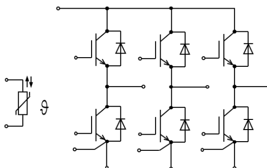
Internal Circuit
